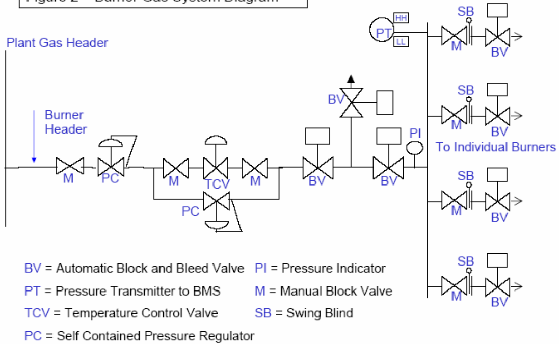
Figure 2 – Burner Gas System Diagram
