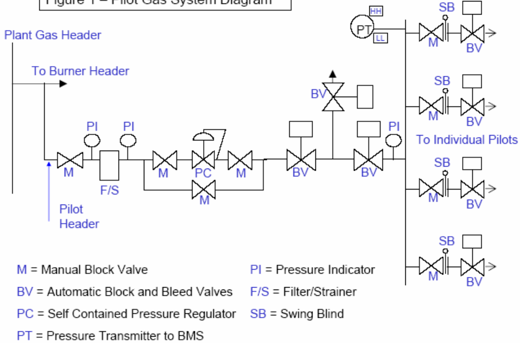
Figure 1 – Pilot Gas System Diagram
